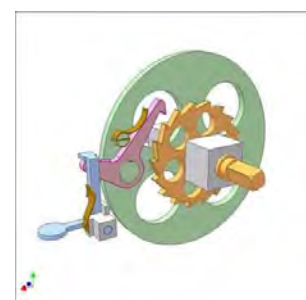
Ratchet 360 degrees
