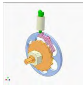
Ratchet clutch
